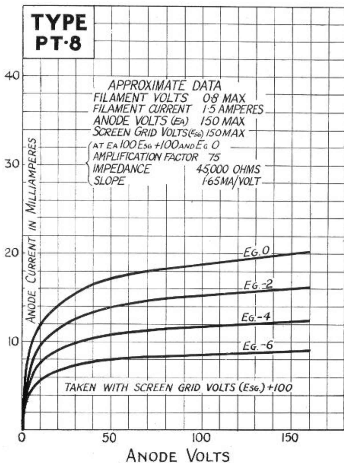
Characteristic Curve of Average PT.8 Valve.
